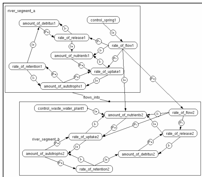
Figure 7: The dependencies of the scenario shown in Figure 4
