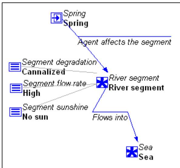
Figure 3: The simplest scenario for a river in our simulation tool composed of a spring, a river segment, and the sea. The river segment here is specified as canalized, high flow rate and no sunshine reaching the river.
