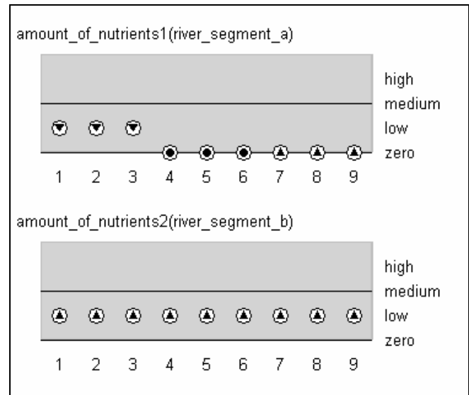
Figure 6: The value history for the variable amount of nutrients in the upstream and the downstream river segment in the scenario shown in Figure 2.
