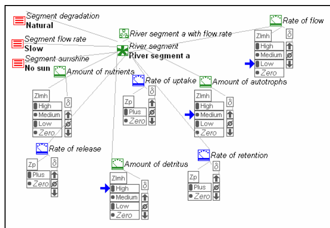
Figure 2: The Model Fragment for a natural, slow flowing river segment which is not reached by much sunlight contains the consequences for the flow rate and the amount of autotrophs and detritus. The value is set by the arrows.
