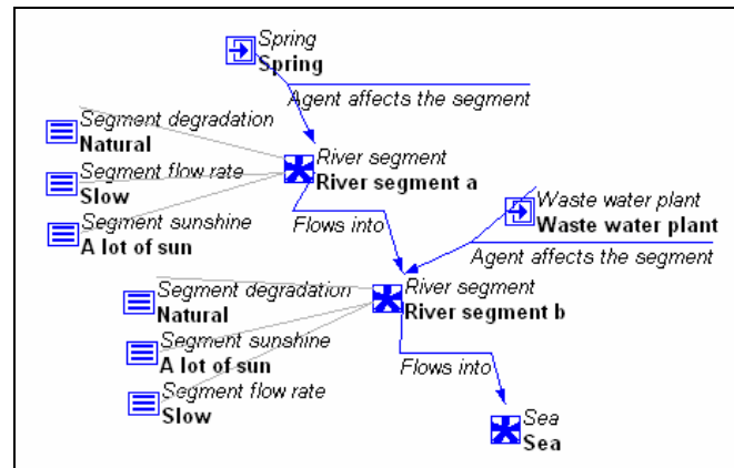
Figure 4: A scenario for a natural stream with slow flow rate and with sunshine. The second river segment is affected by a waste water plant.
